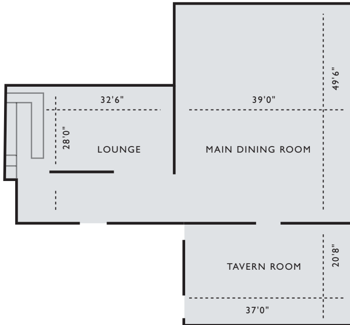
MAIN DINING FLOOR PLAN
